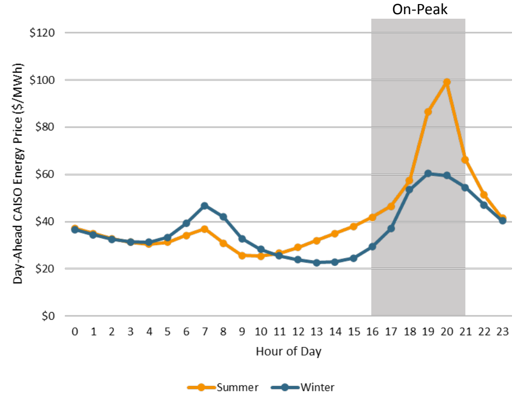
Average Energy Prices by Hour from 2018–2020
