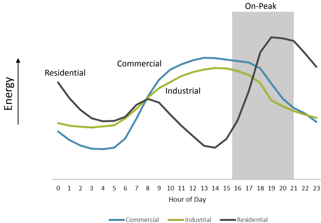
Representative Class Daily Load Shapes
